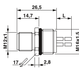
Dimensions: plug
