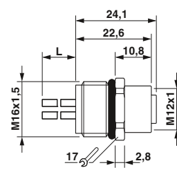
Dimensions: socket
